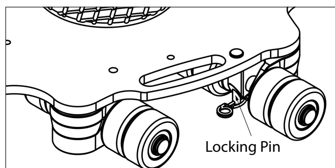
Figure 7: MLSR locking mechanism detailed view
