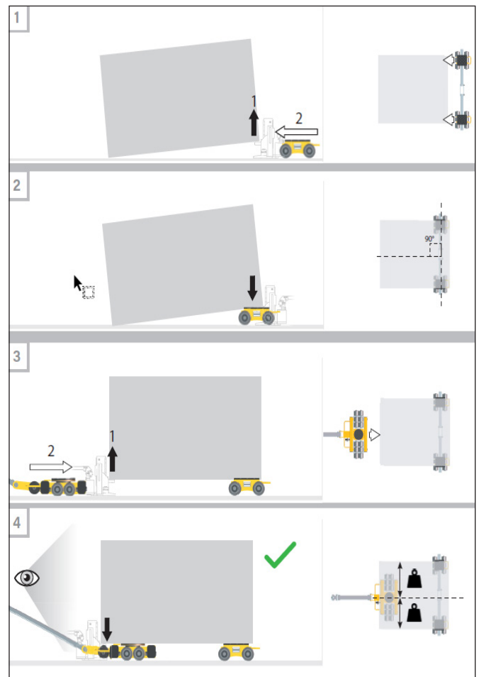
Figure 8: Lifting process
