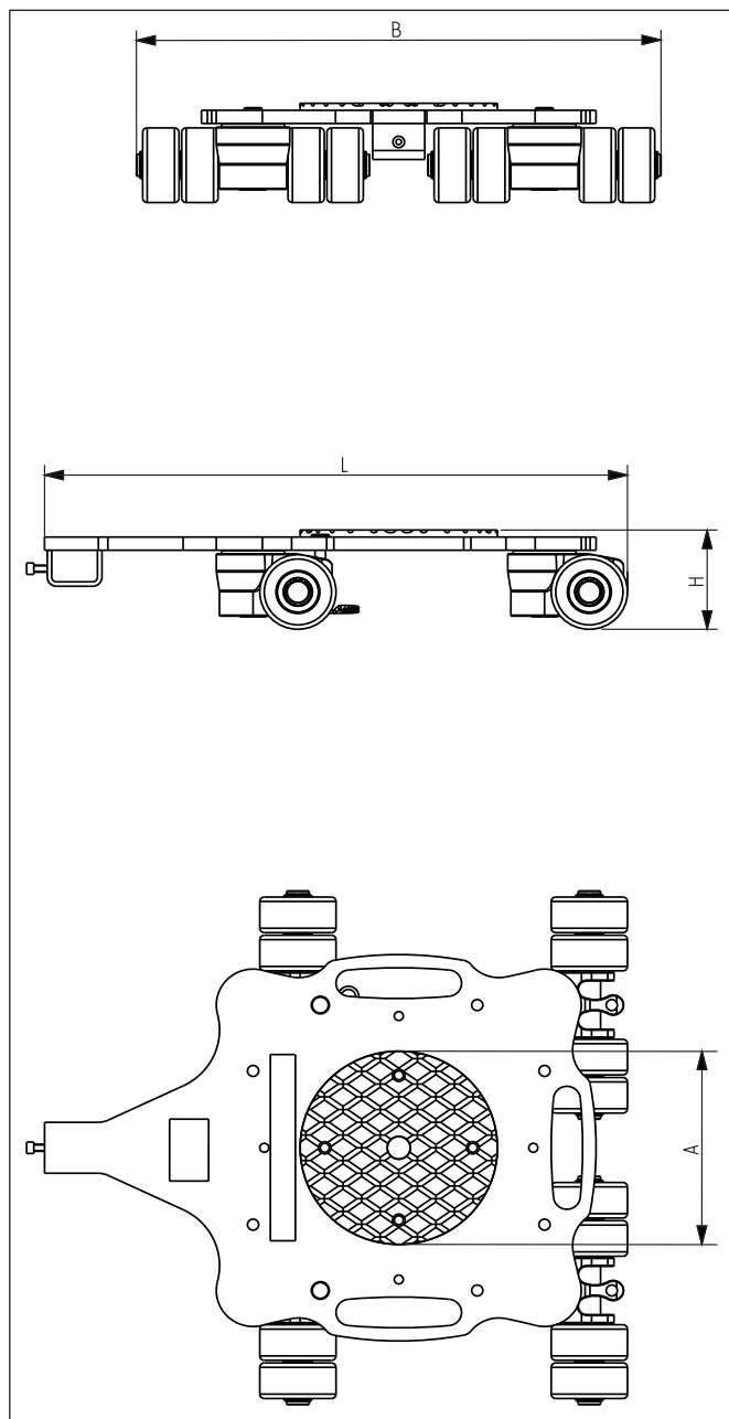
Figure 6: MLSR load skate dimensions
