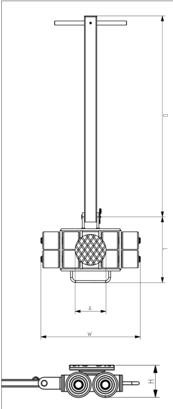
Figure 4: MLSF load skate dimensions
