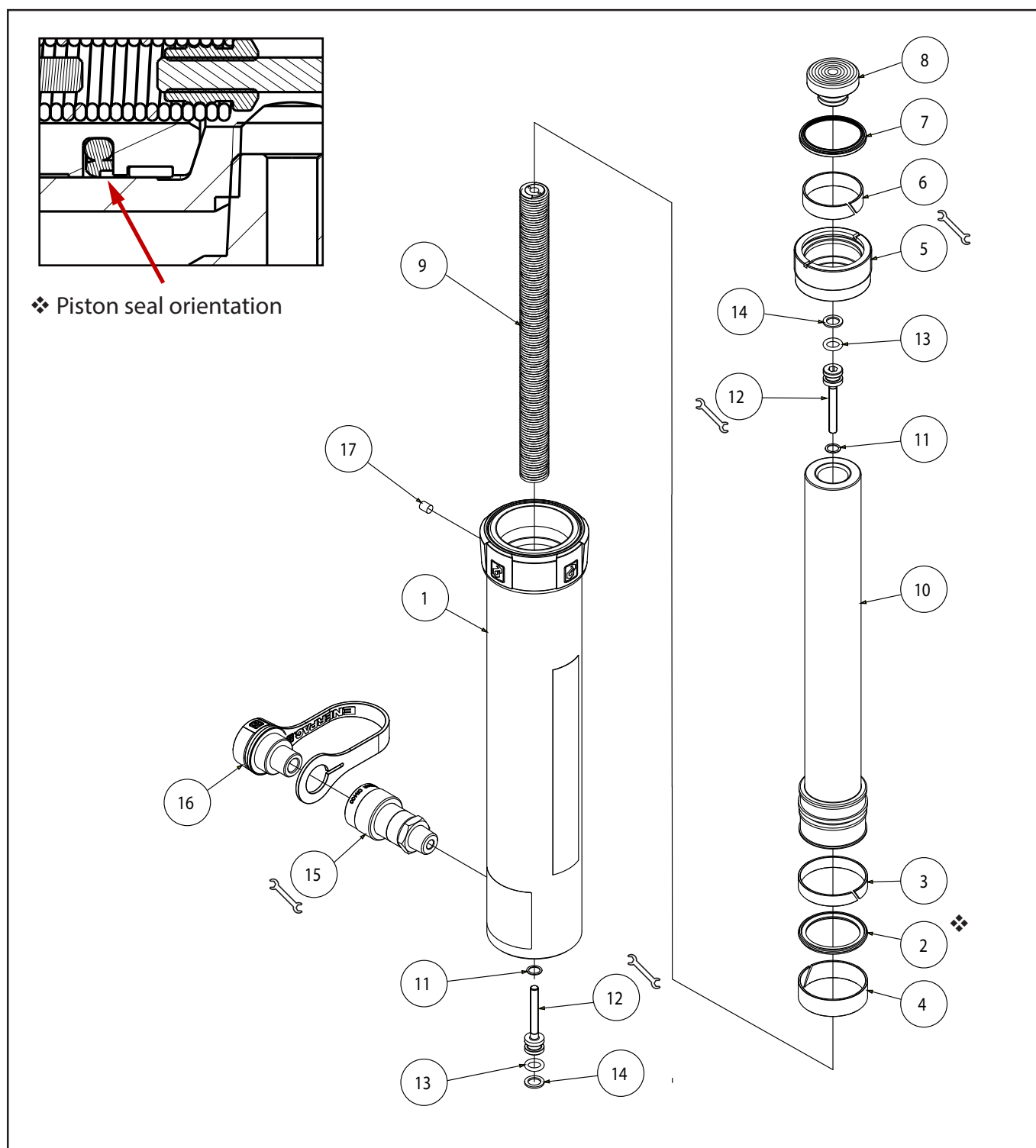
Figure 1, RC Hydraulic Cylinder, 15 Ton
