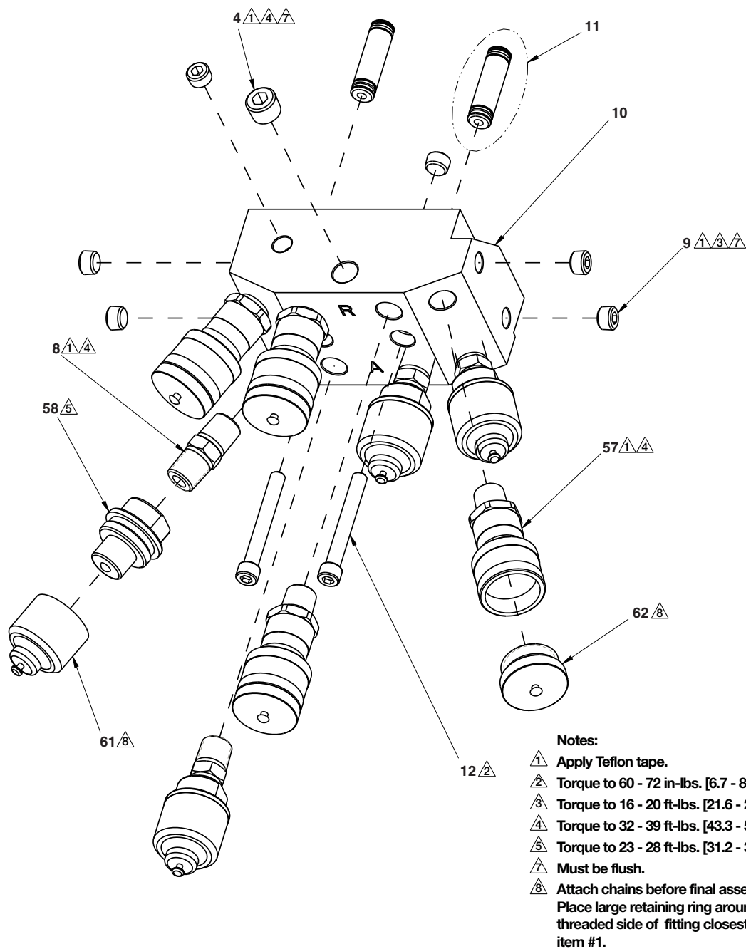
Figure 6, TQM Multi Port Manifold Assembly (optional)
