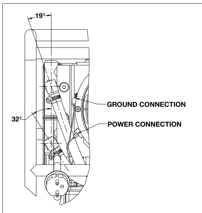
Figure 2B, Oil Cooler Wiring Details
