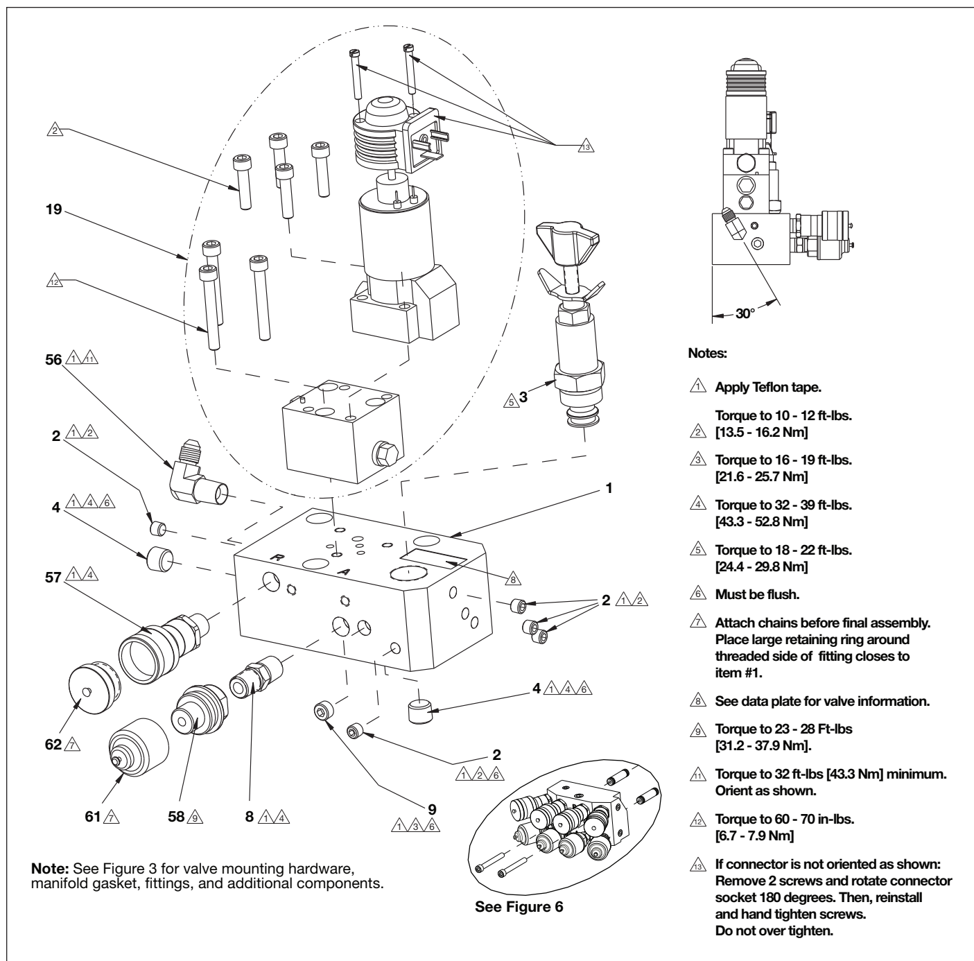
Figure 5, Control Valve Assembly
