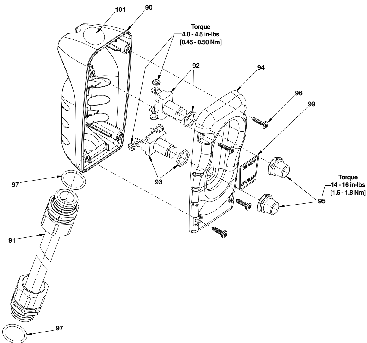
Figure 10, Pendant Assembly, 2-Button
