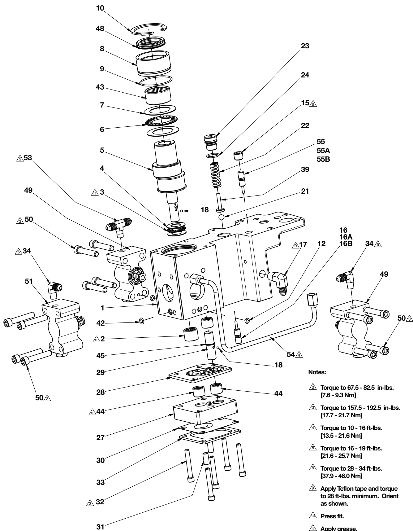
Figure 8A, Pump Element Assembly, DD2693900SR
