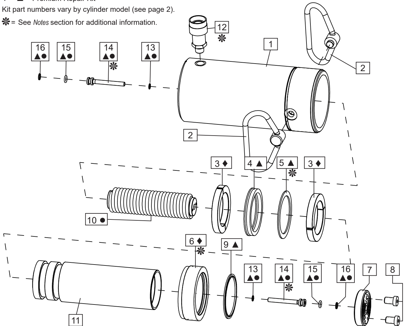
Fig. 1, Cylinder Assembly
