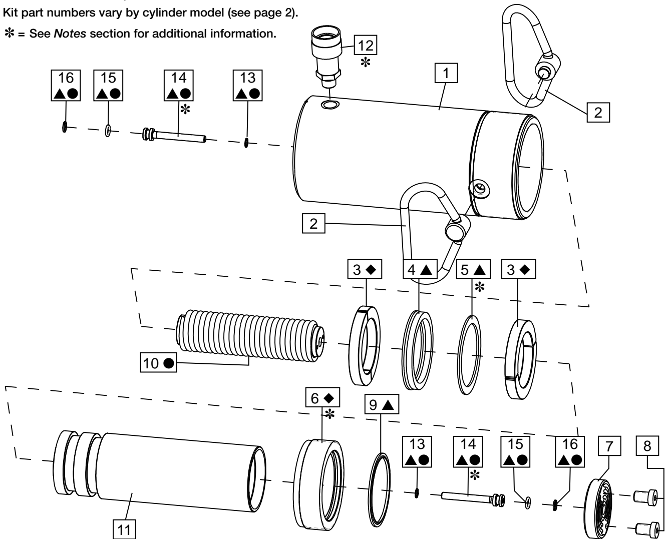
Fig. 1, Cylinder Assembly
