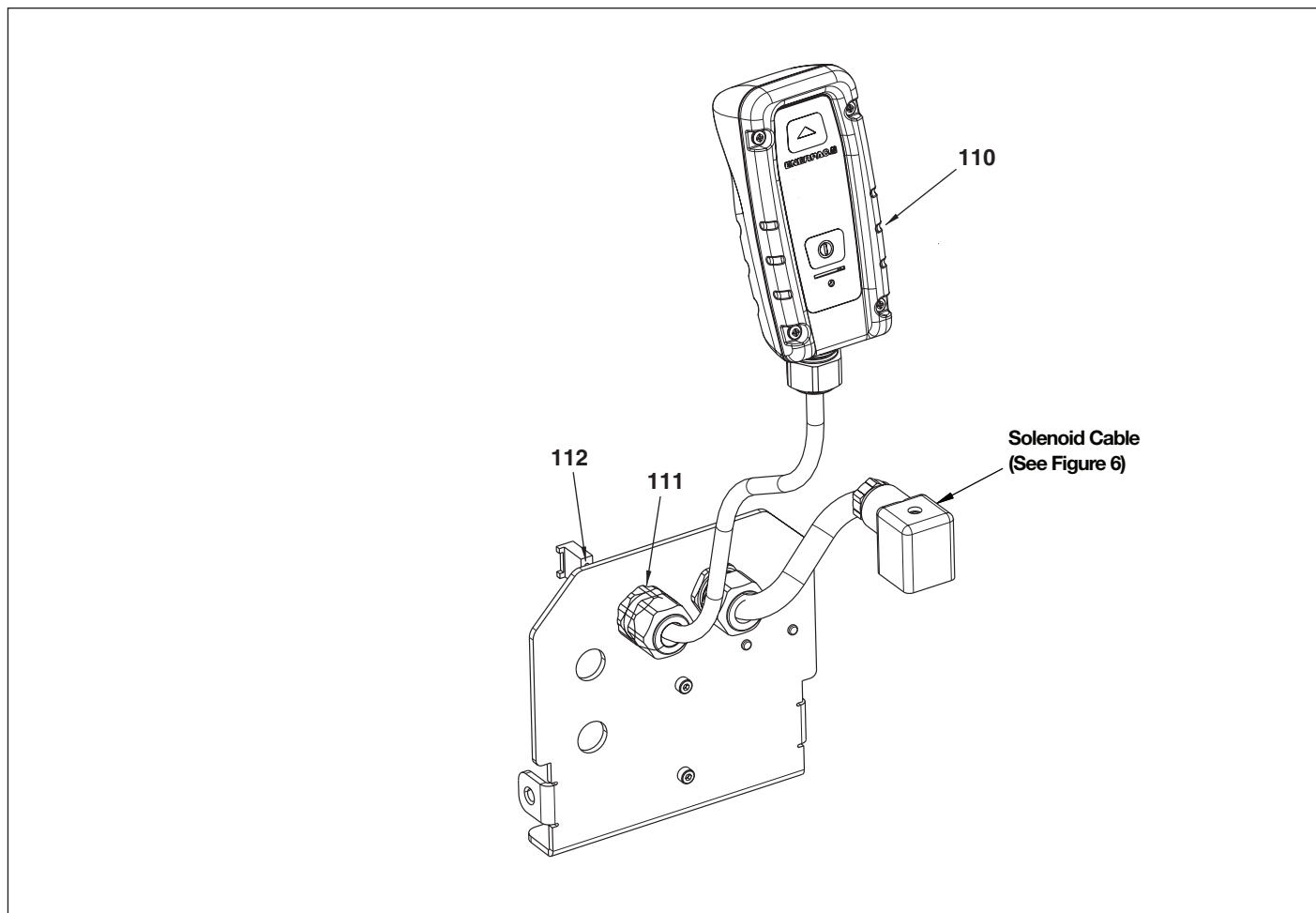
Figure 8, Pendant Assembly
