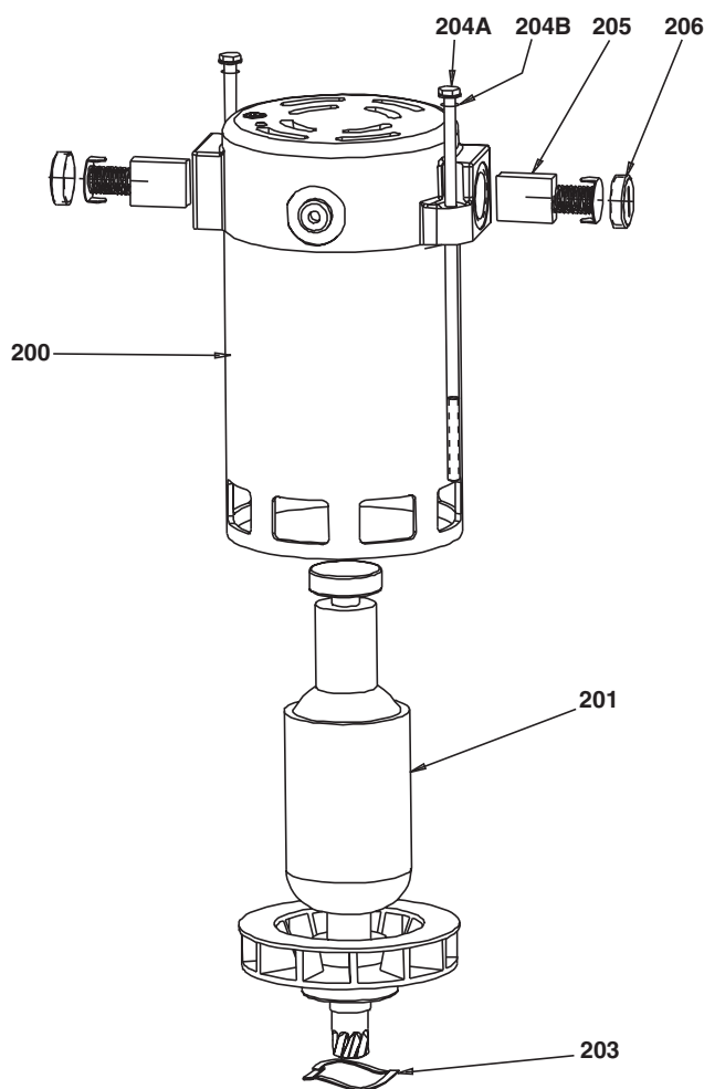
Figure 10, Motor Assembly
