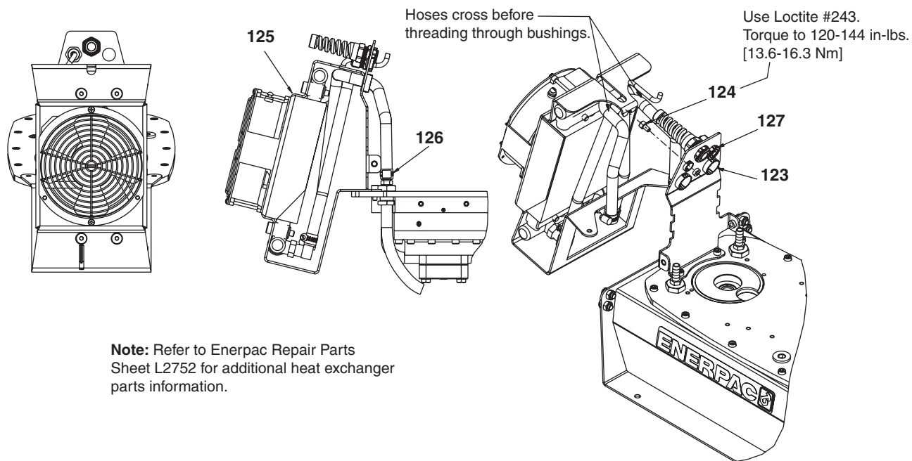
Figure 9, Heat Exchanger, 115 and 230 VAC Fan
