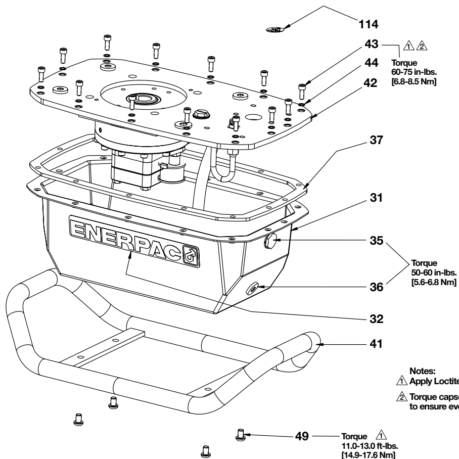
Figure 1, Reservoir Assembly
