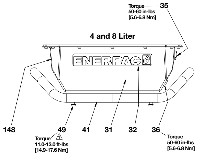
Figure 1, Reservoir Assembly
