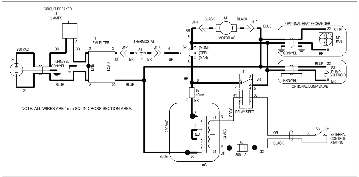
Figure 15, Electrical Schematic, 230V Models
