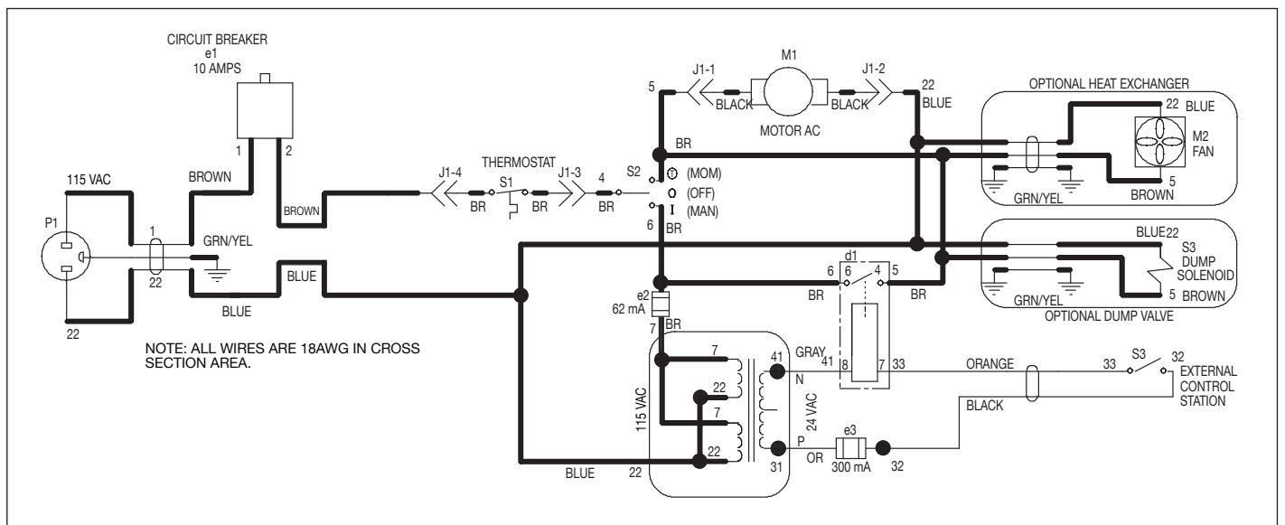
Figure 14, Electrical Schematic, 115V Models
