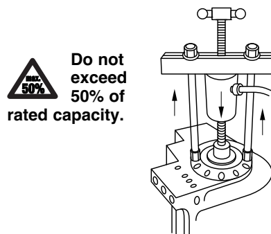
illustration 3 - Pushing with cross bearing puller
