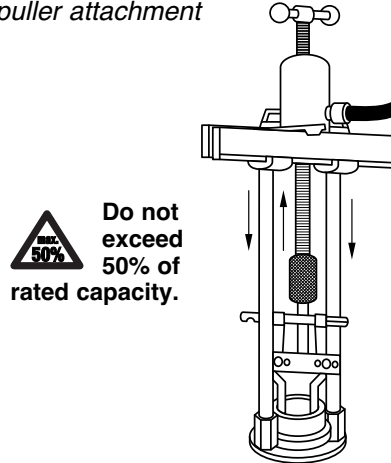
illustration 2 - Crosshead puller with bearing cup puller attachment
