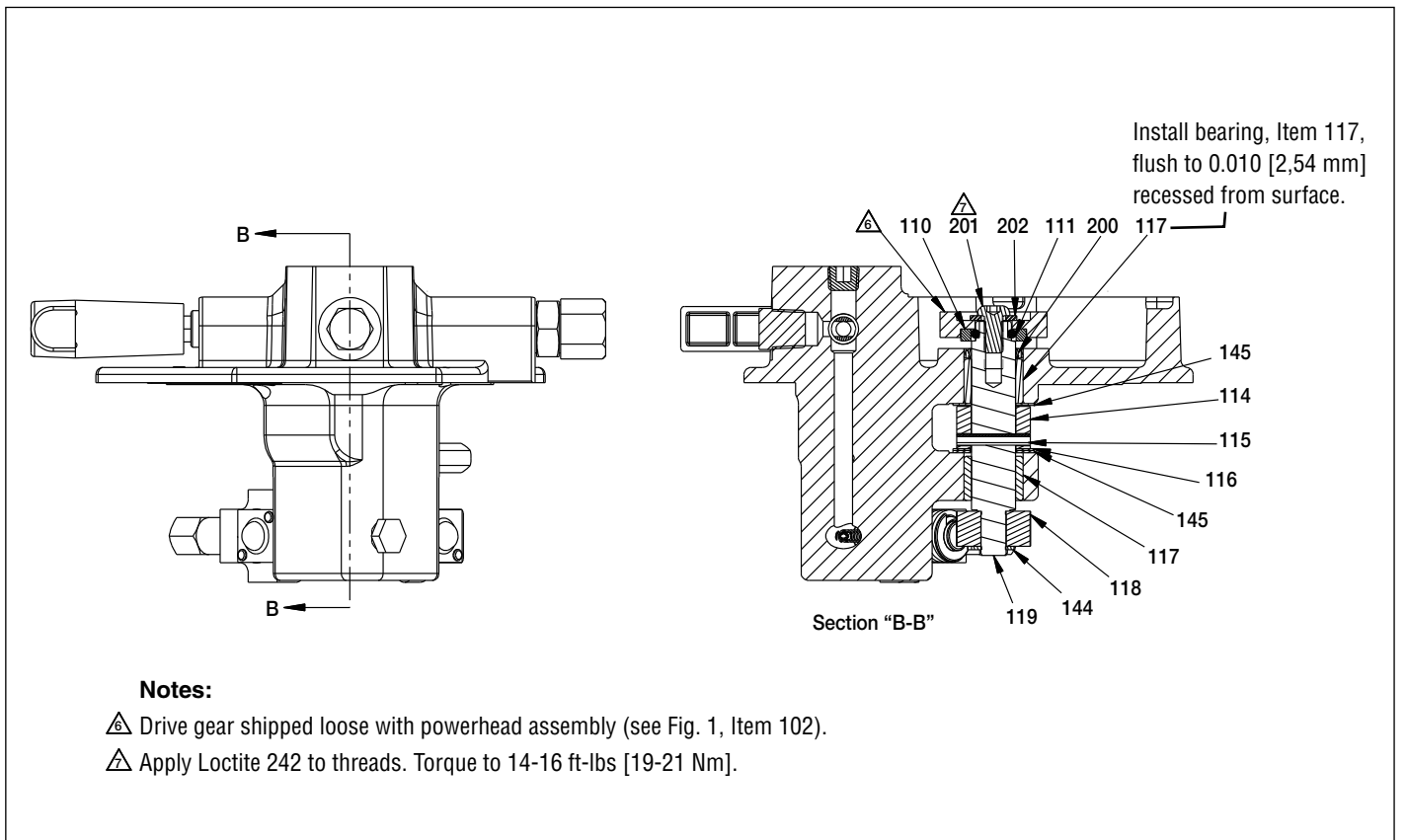
Figure 4, Pump Shaft Details
