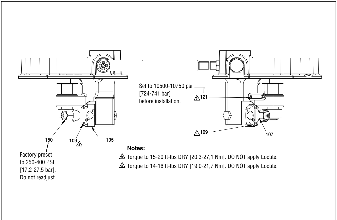
Figure 5, Piston Block Assemblies
