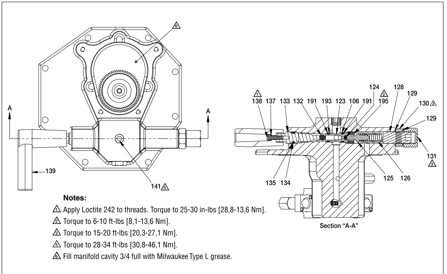
Figure 3, Valve And Mainfold Assy
