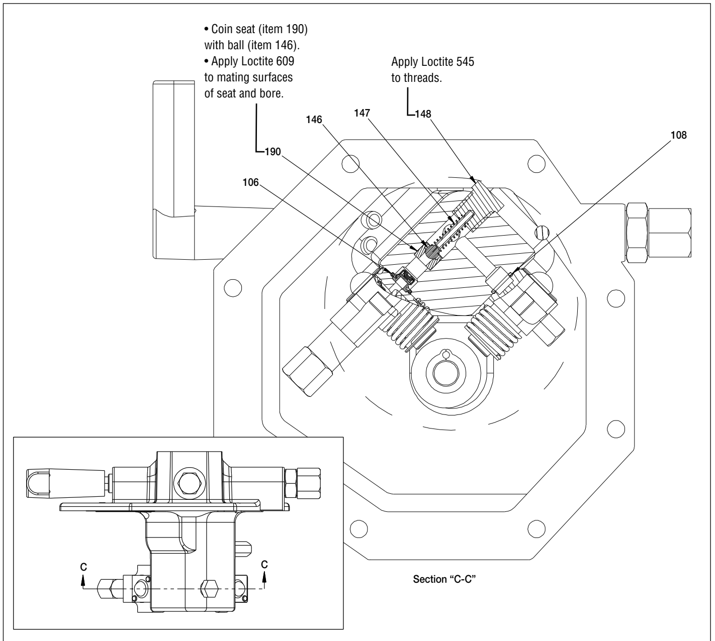
Figure 6, Pump Check Ball Assembly (bottom view)
