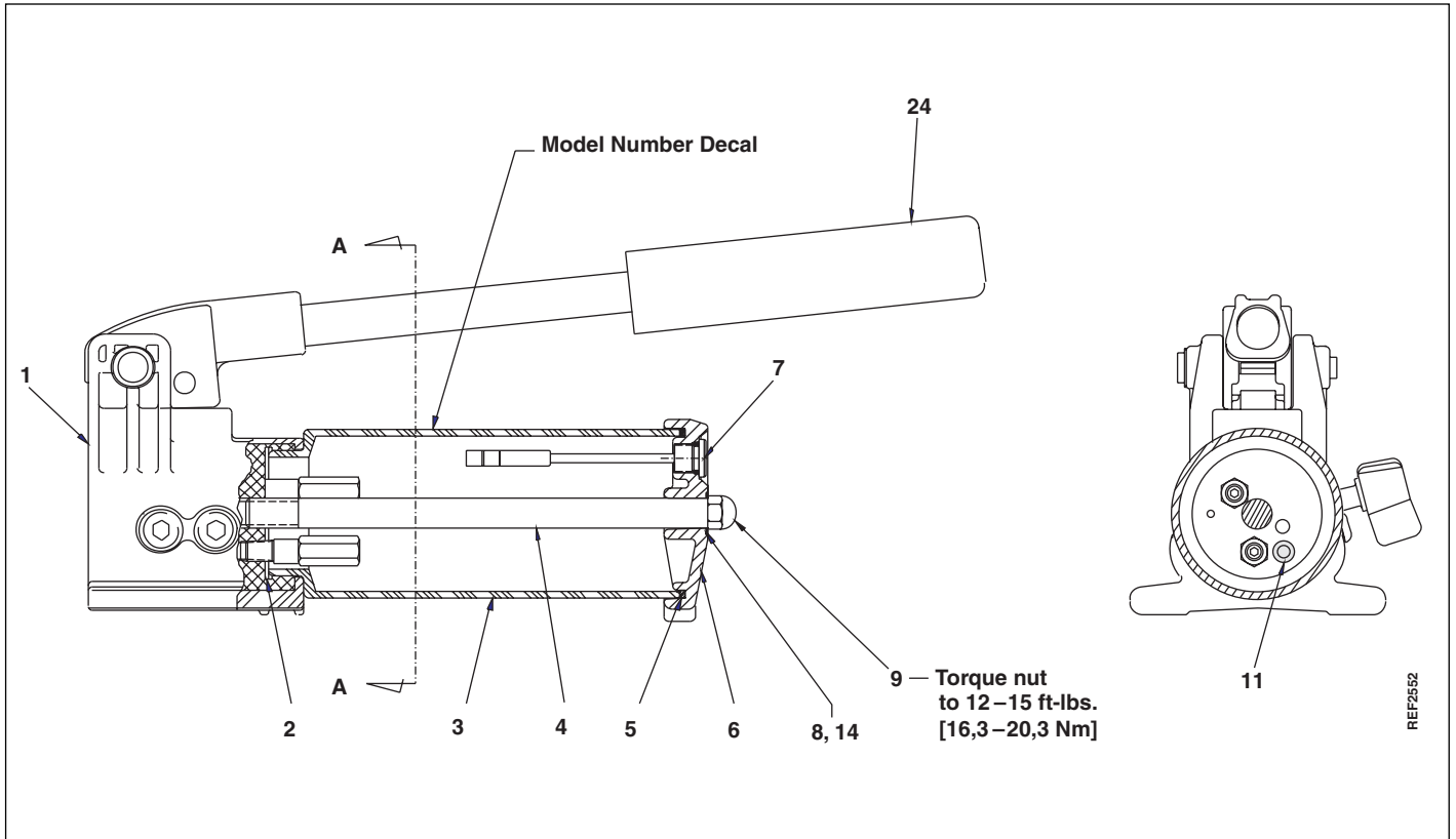
Figure 1, Pump Assembly
