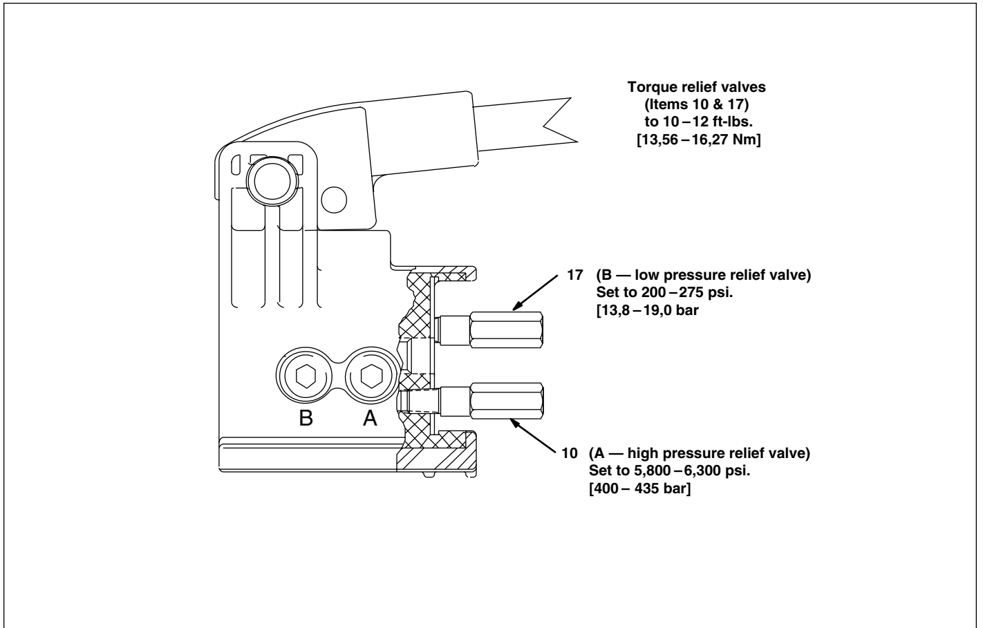
Figure 3, Pumping Unit Assembly
